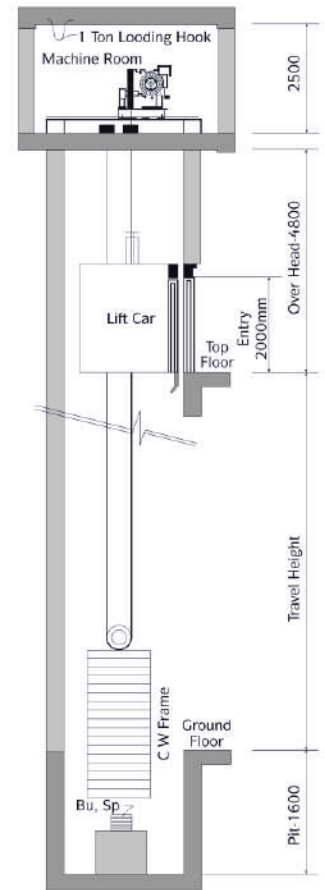
(section : X-X) Lift Well
