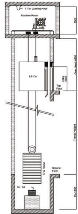
(section :X-X) Lift Well
